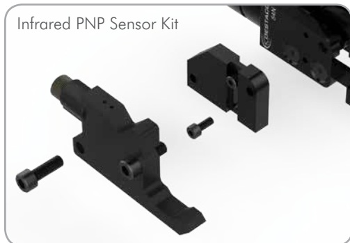
Sheet Stop
