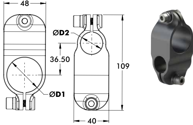
Ø40mm/1.50 in to Ø25mm/1.00 in Cross Clamp
